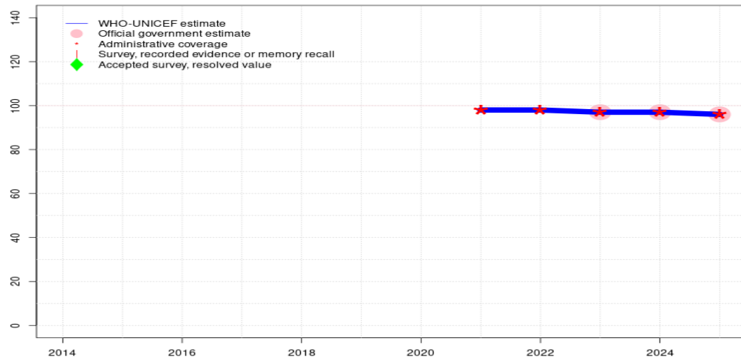
ALB - IPV1C
